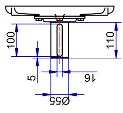
Shaft detail
