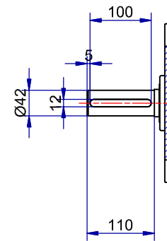
Shaft detail
