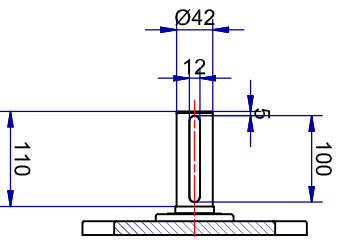
Shaft detail
