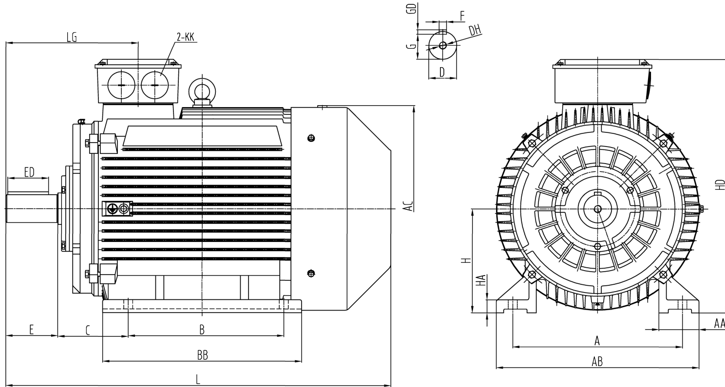
OUTLINE DIMENSIONS FOOT MOUNTED MOTORS
