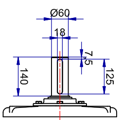
Shaft detail
