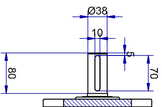
Shaft detail
