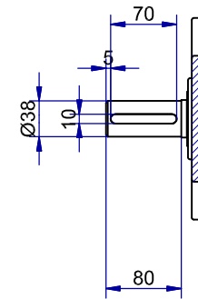
Shaft detail
