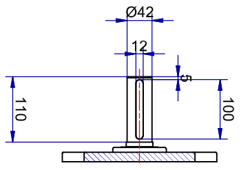
Shaft detail
